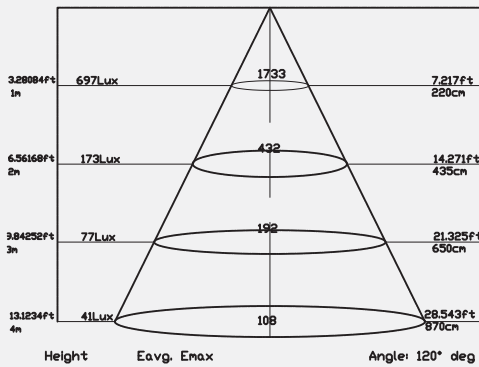
Photometry 2800K
