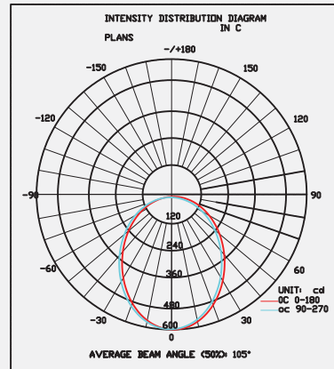
Photometry 4000K
