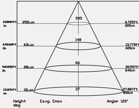
Photometry 4000K
