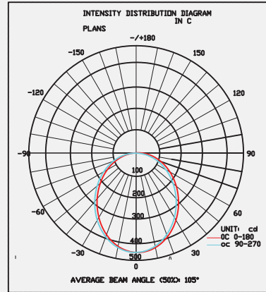
Photometry 2800K
