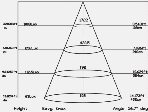
Photometry 60°
