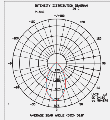
Photometry 60°
