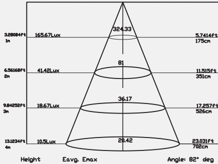
Photometry 100°
