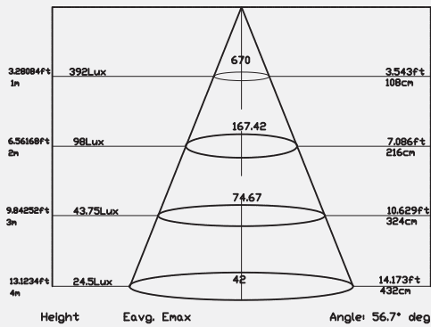
Photometry 60°
