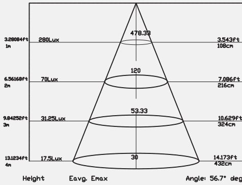
Photometry 60°
