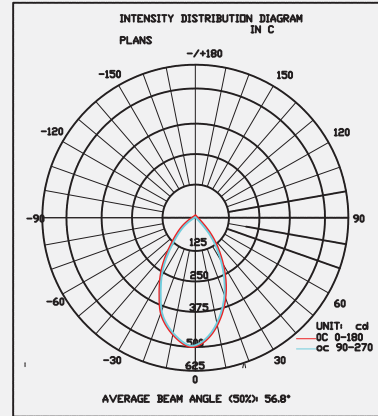
Photometry 60°
