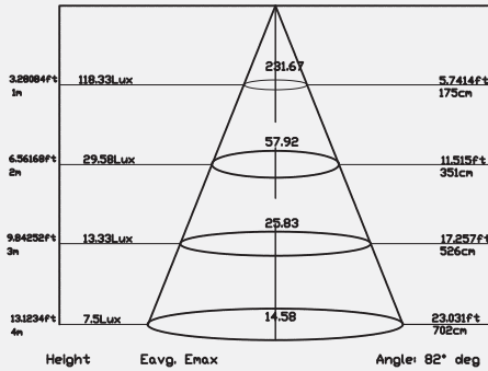
Photometry 100°
