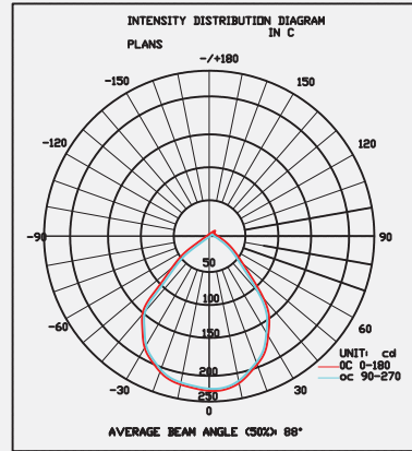
Photometry 100°
