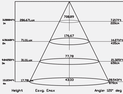
Photometry 2800K
