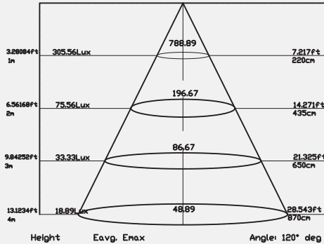
Photometry 4000K
