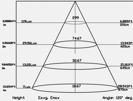
Photometry 4000K
