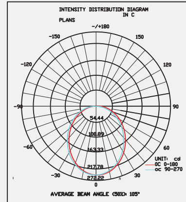
Photometry 2800K
